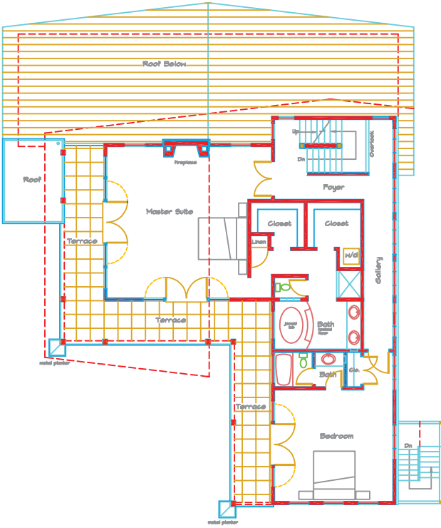
MBR LEVEL PLAN north scale: 1/4" = 1'-0" area hvls: 1480 SF
