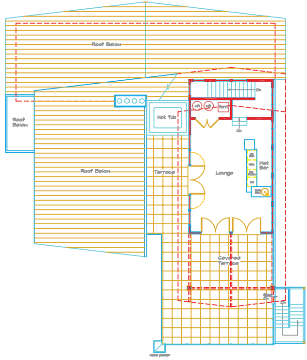
LOUNGE-TERRACE LEVEL PLAN north scale: 1/4" = 1'-0" area hvls: 549 SF
