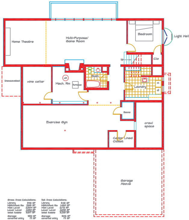
LOWER LEVEL PLAN north scale: 1/4" = 1'-0" area hvls: 2219 SF
