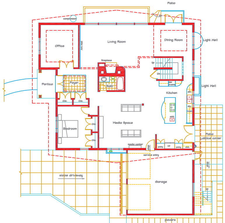
MAIN LEVEL PLAN north scale: 1/4" = 1'-0" area hvls: 2772 SF
